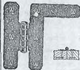
FOR 3/8 INCH FLUSH DOORS
