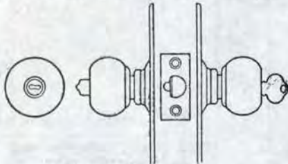
Guarded Latch Bolt
